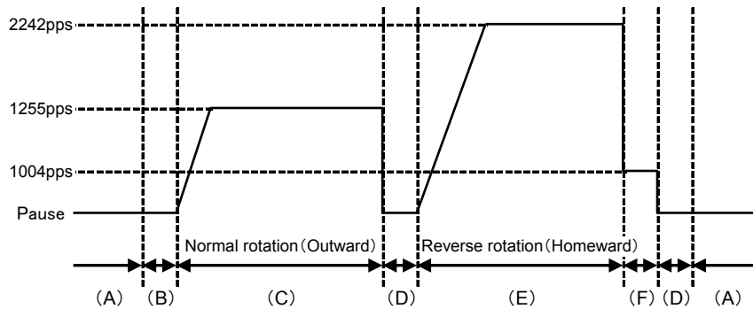
Figure 5-3 Timing Chart for Autocutter Drive (CAPD245)
