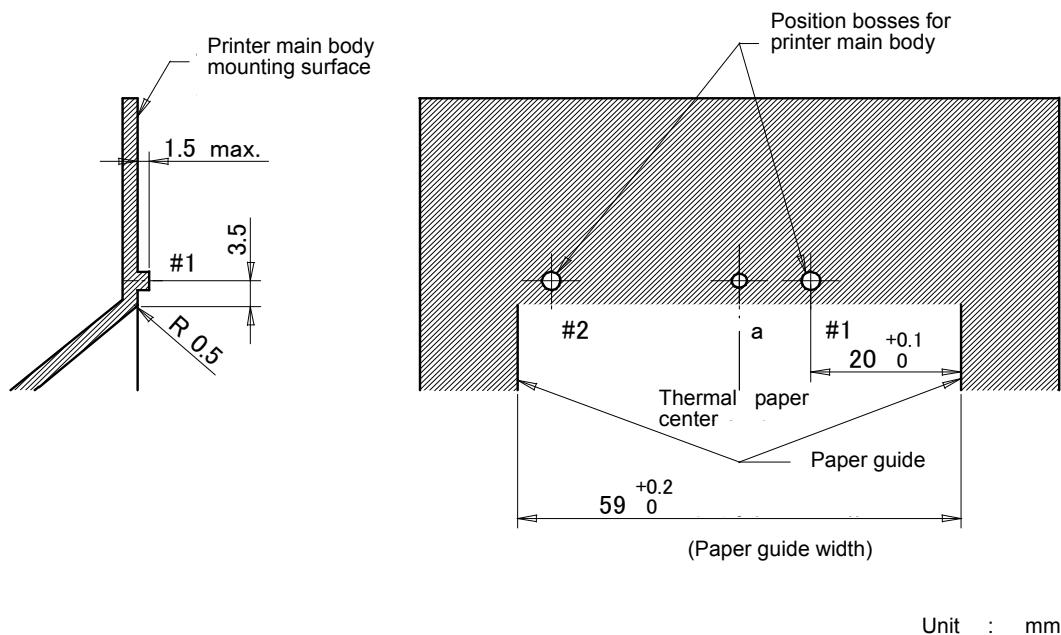
Figure 6-11 Recommended Paper Holder Dimensions
