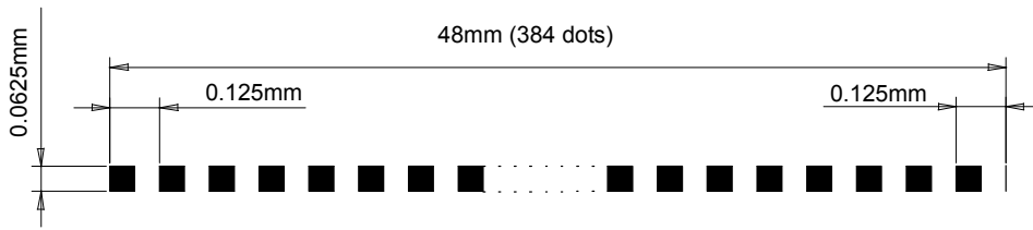
Figure 3-1 Dot Pitch
