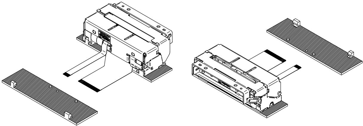
Figure 6-3 Sample for Positioning and Securing the Printer Main Body (1) (Fixed by the Mounting Part a, b and b')
