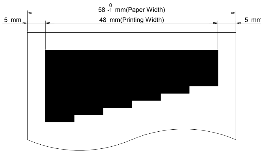
Figure 3-2 Print Area
