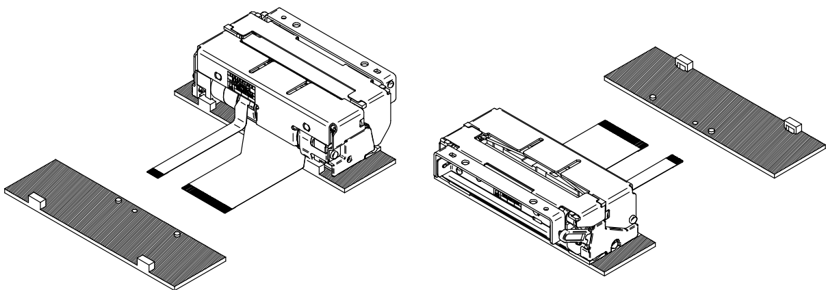
Figure 6-5 Sample for Positioning and Securing the Printer Main Body (3) (Fixed by the Mounting Part a, c and c')
