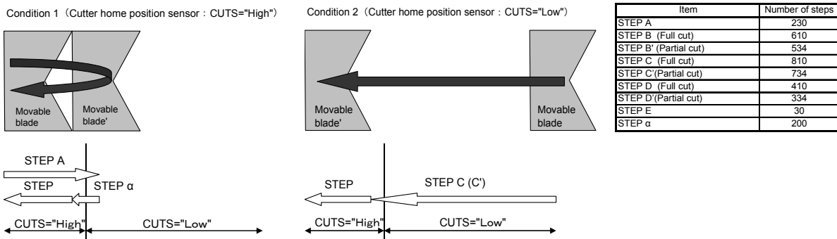
Figure 5-4 Autocutter Flow Chart : Initializing
