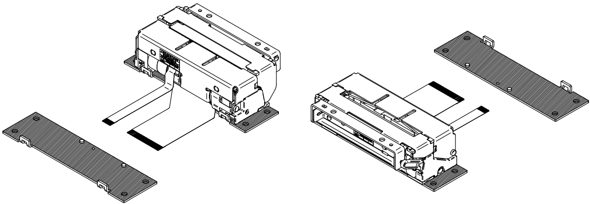
Figure 6-4 Sample for Positioning and Securing the Printer Main Body (2) (Fixed by the Mounting Part a, c and c')
