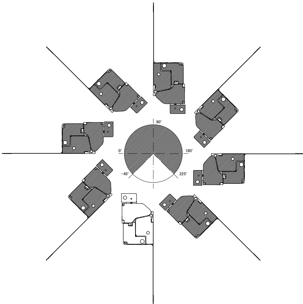
Figure 6-1 Mounting Position
